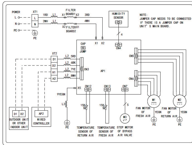
Internal wiring diagram of FHBQGL-D5DA-T Fig 8 Internal wiring diagram
