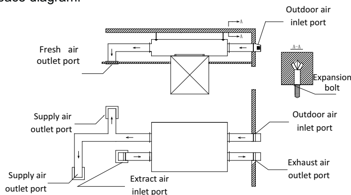
Fig 5 Installation diagram
