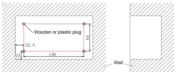
Fig.3.8 Diagram of Wooden or Plastic Plug
