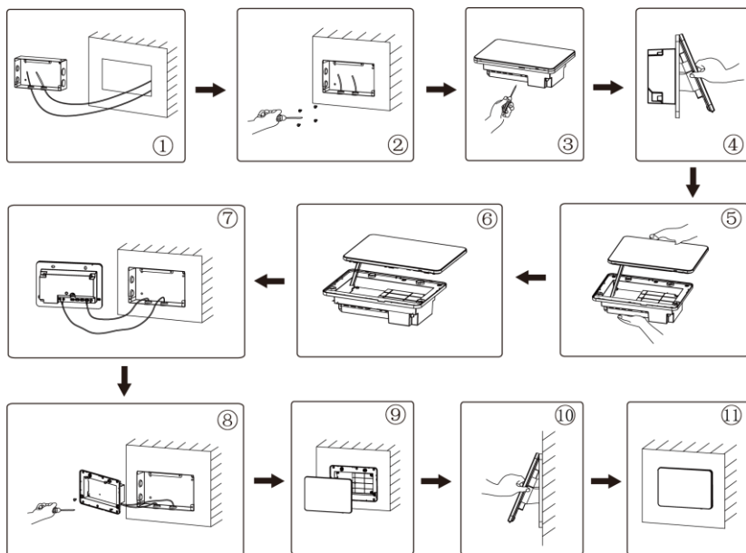
Fig.3.7 Installation Diagram
