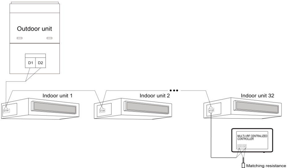
Fig.3.4 Centralized Controller Connected with Indoor Network
