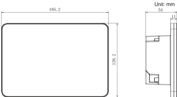
Fig.3.2 Dimension of Centralized Controller
