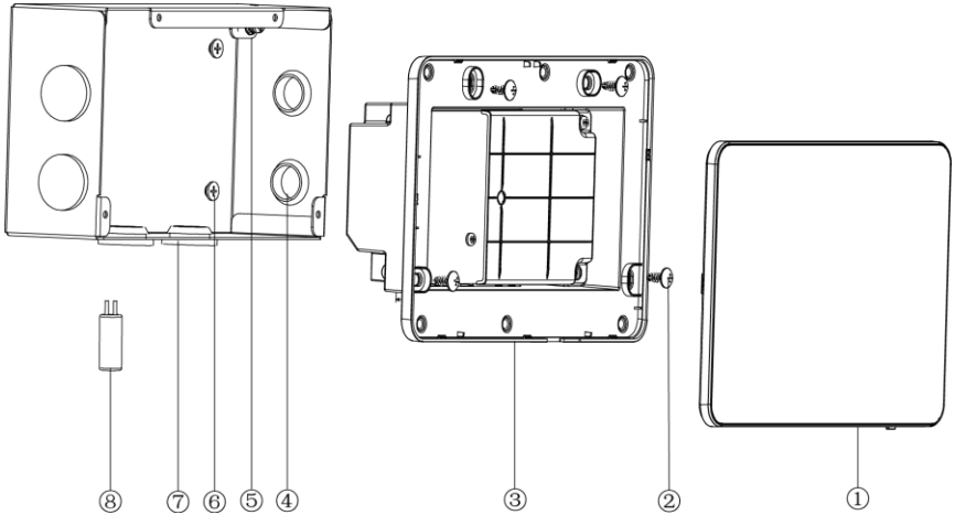
Fig.3.1 Parts of Centralized Controller
