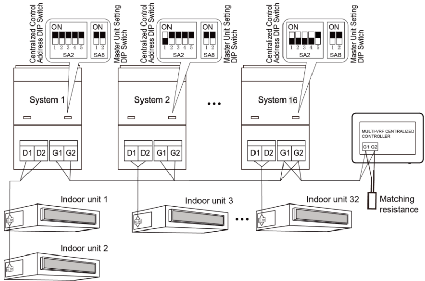
Fig.3.5 Centralized Controller Connected with Outdoor Network
