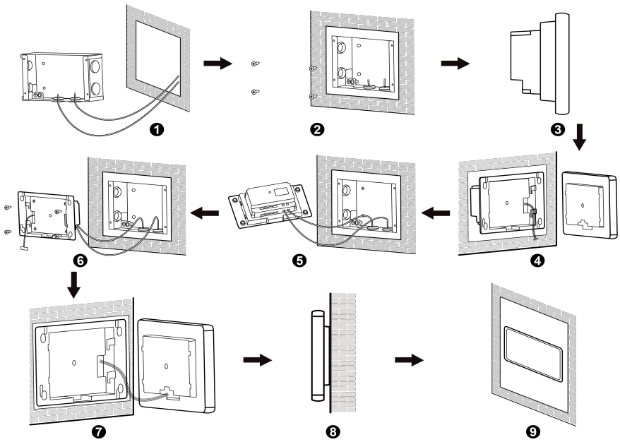
Fig. 3.11 Installation
