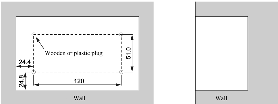
Fig. 3.12 Wooden wedge or plastic wedge
