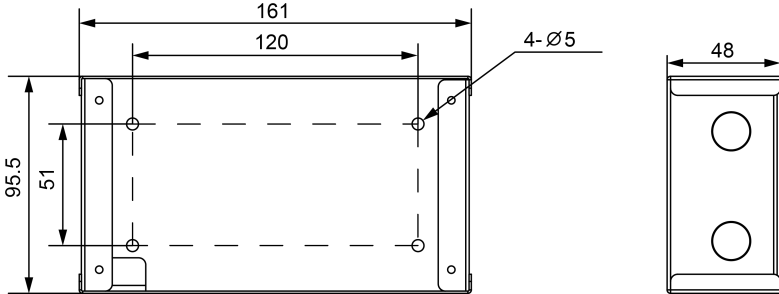
Fig. 3.3 Dimension of Electric Box
