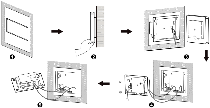
Fig. 3.14 Disassembly
