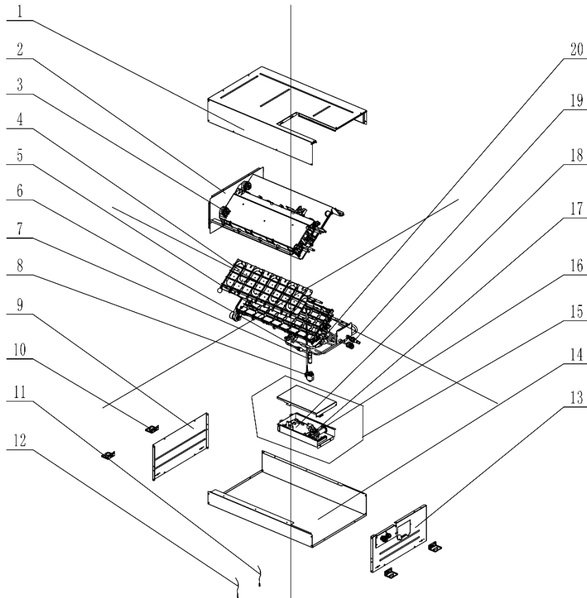
Exploded View of XRZ180L/A-T
