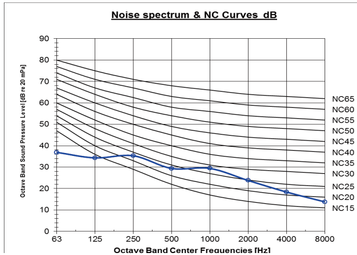
Model GMV-ND50~63PLS/B1-T
