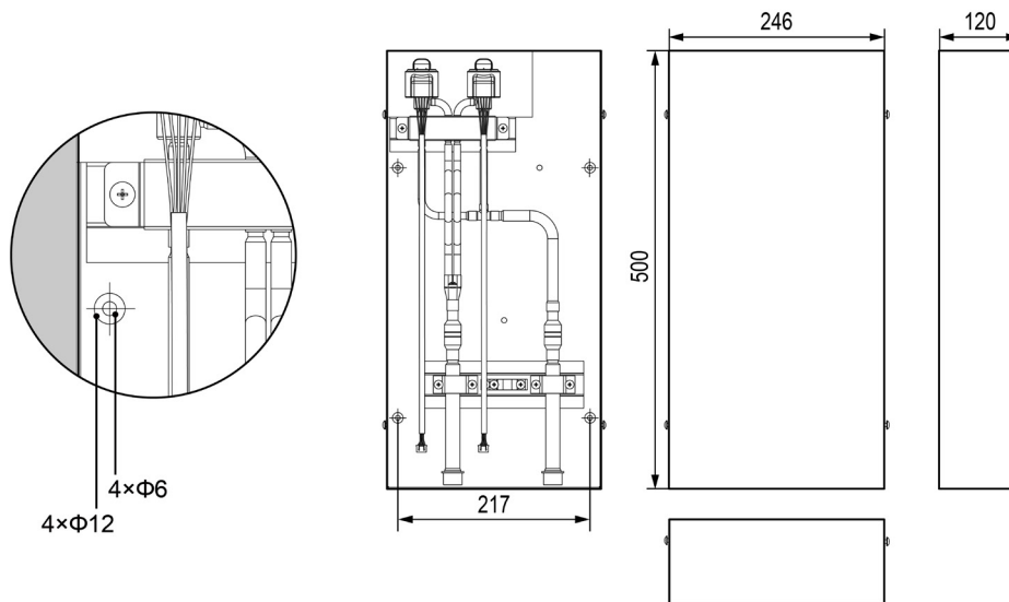
(4) Size of EXV box for GMV-N560U/A-T (Unit: mm):
