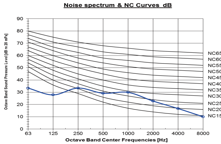
Model GMV-ND50~63PLS/B1-T
