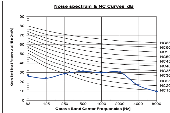
Model GMV-ND22~28PLS/B1-T
