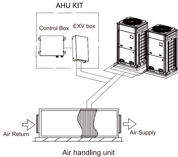
AHU-KIT one-to-one (combination outdoor unit) connection diagram
