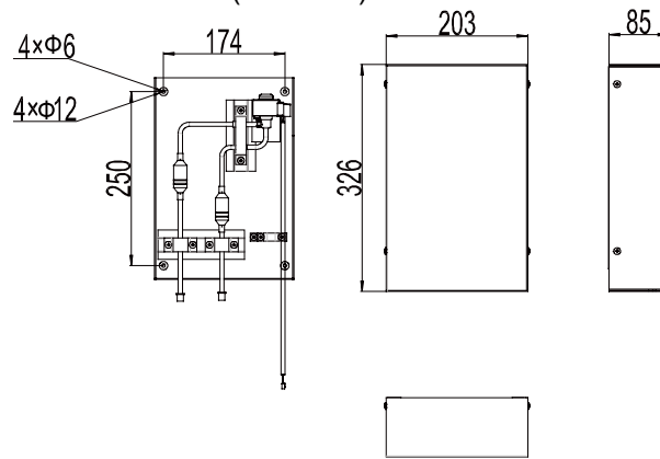
(2) Size of EXV box for GMV-N36U/C-T(Unit: mm):
