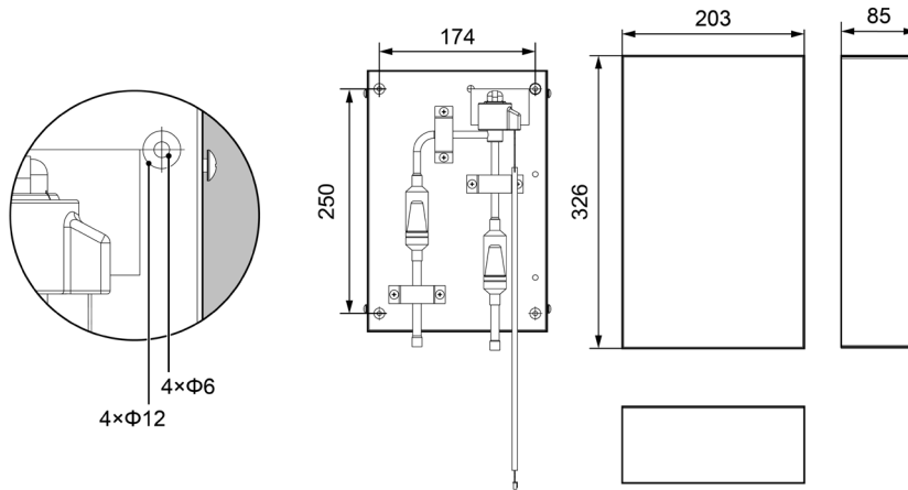
(4) Size of EXV box for GMV-N560U/A-T (Unit: mm):
