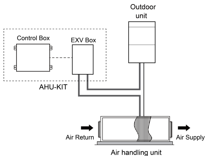
AHU-KIT one-to-one (single unit) connection diagram
