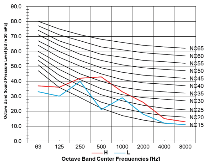
Noise spectrum & NC Curves dB
