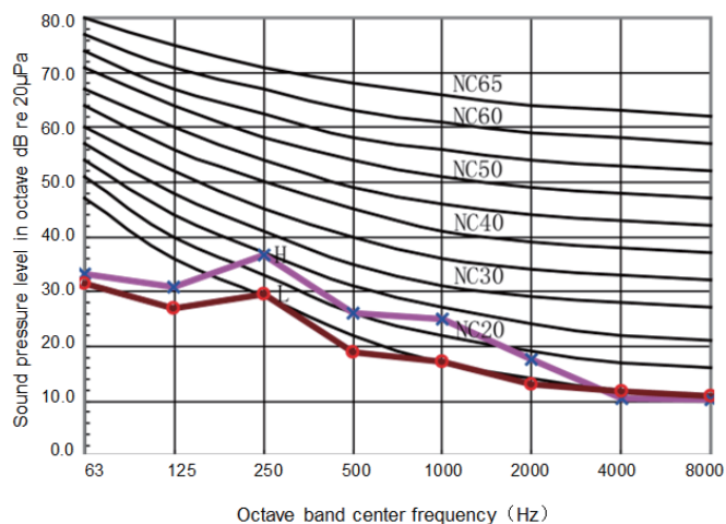
Model GMV-ND40~50PLS/K-T
