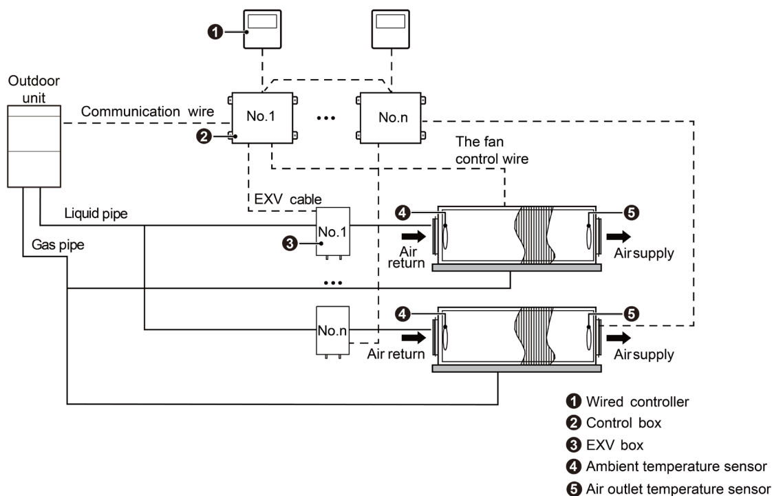
GMV one-to-multiple AHU-KIT connection (2.8kW≤capacity≤168kW)
