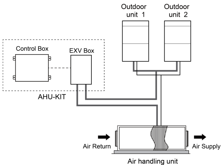
AHU-KIT one-to-one (combination outdoor unit) connection diagram
