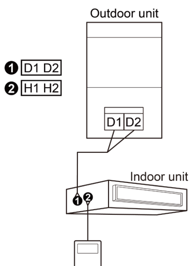
One wire controller controls one indoor unit
