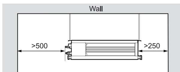
(2) Slim Duct Type GMV-ND**PL/B-T Series
