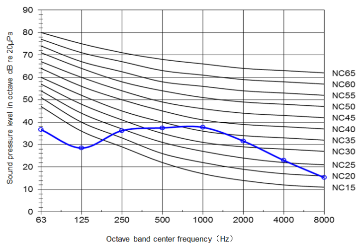
Model GMV-ND40~45PLS/B1-T
