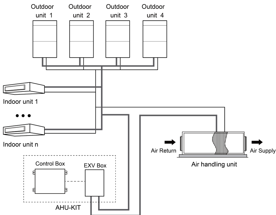
AHU-KIT one-to-more (hybrid connection) connection diagram
