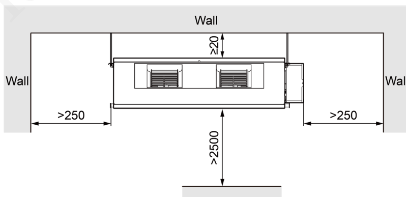
(4) Super High Static Pressure Duct Type Indoor Unit GMV-ND**PHS/B-T Series
