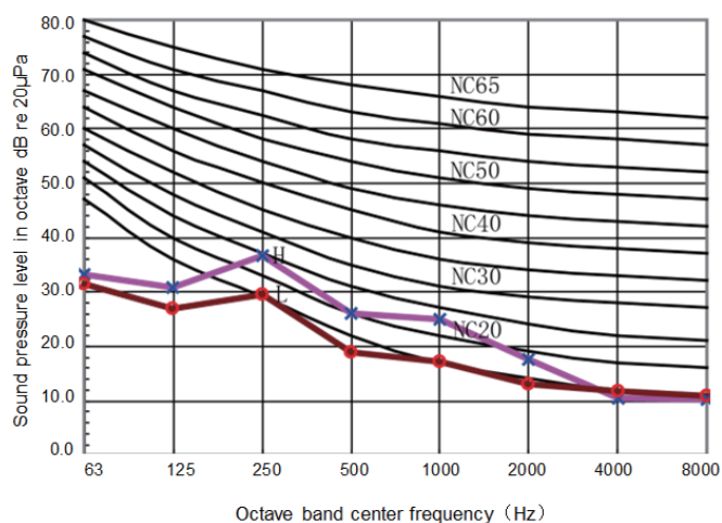
Model GMV-ND40~50PLS/K-T
