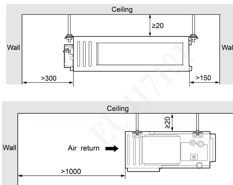
(4) Super High Static Pressure Duct Type Indoor Unit GMV-ND**PHS/B-T Series
