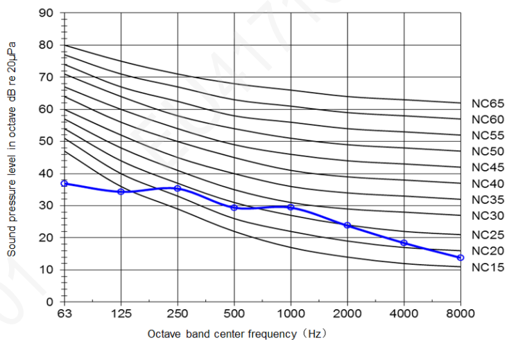
Model GMV-ND71PLS/B1-T
