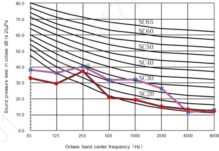
Model GMV-ND56~63PL/B-T
