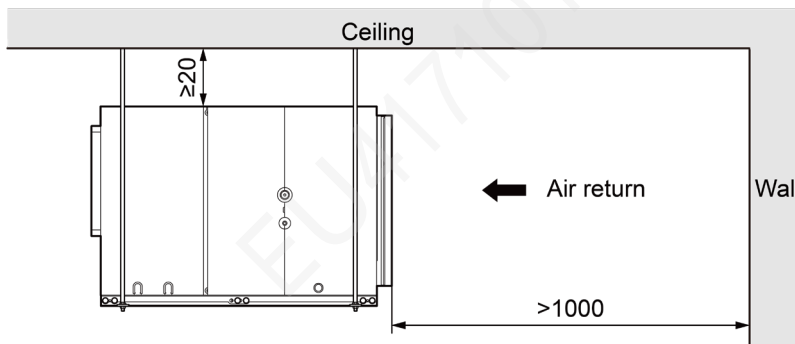
GMV-ND450PH/AR-X
