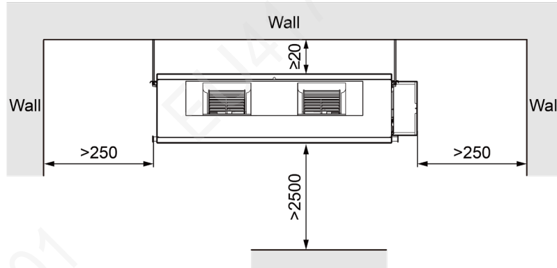
(4) Super High Static Pressure Duct Type Indoor Unit GMV-ND**PHS/B-T Series
