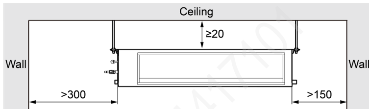
(7) Middle Static Pressure Duct Type Indoor Unit GMV-ND**PMS/A1-T Series
