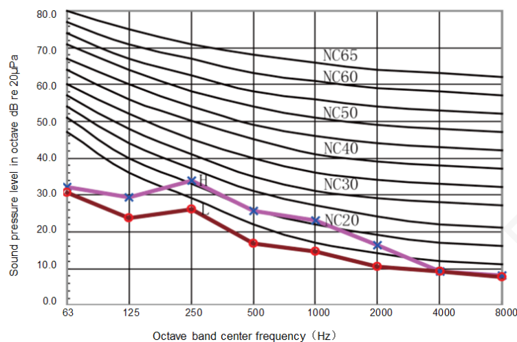
Model GMV-ND32~36PL/B-T
