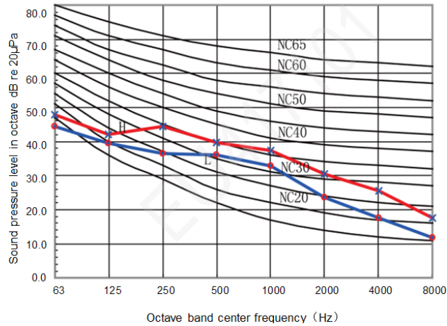
Model GMV-ND125~140PLS/C-T
