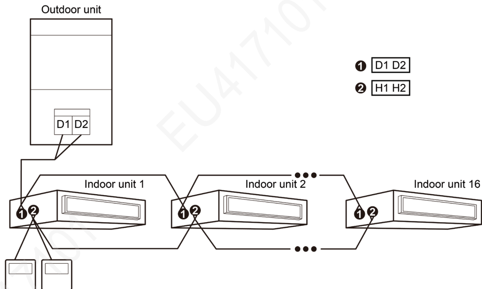
Figure 4 One Receiver and One Wired Controller Control Several Multi VRF IDUs Simultaneously Notes:
