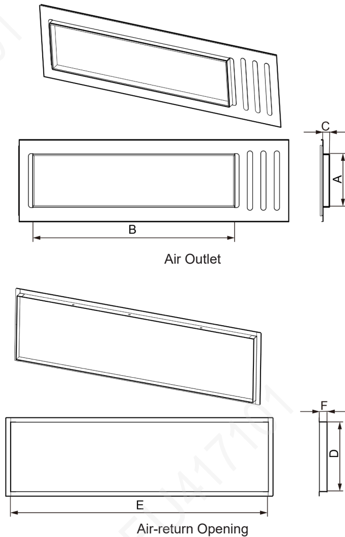
(2) Super High Static Pressure Duct Type Indoor Unit
