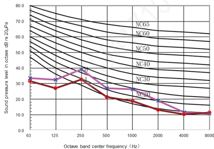
Model GMV-ND32~36PL/B-T
