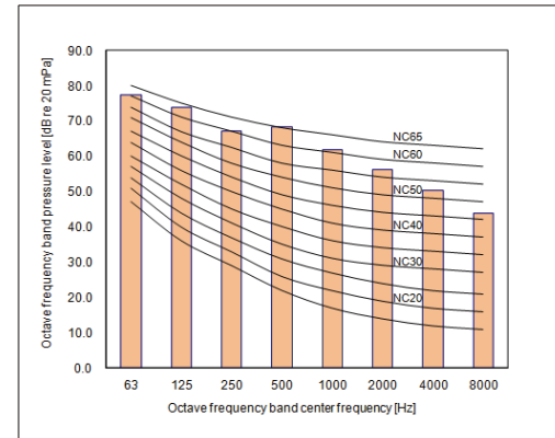
GMV-VQ615WM/C-X
