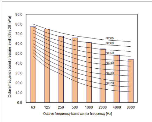
GMV-VQ560WM/C-X
