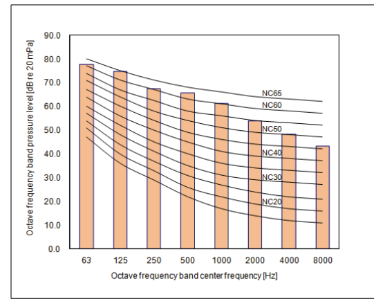
GMV-VQ615WM/C-X
