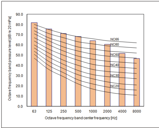
GMV-VQ560WM/C-X
