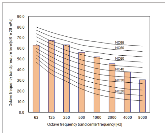
GMV-VQ224WM/C-X
