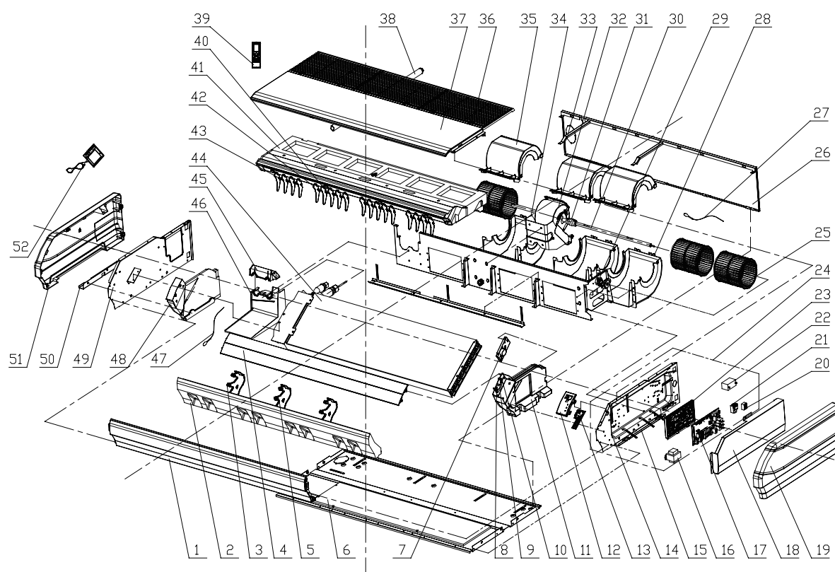
Model:GTH42K3CI exploded view and spare parts list.
