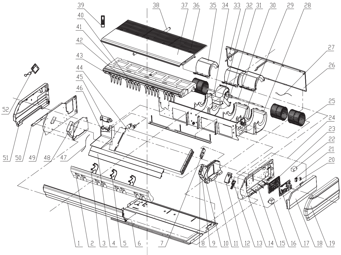
Model:GTH36K3CI exploded view and spare parts list.
