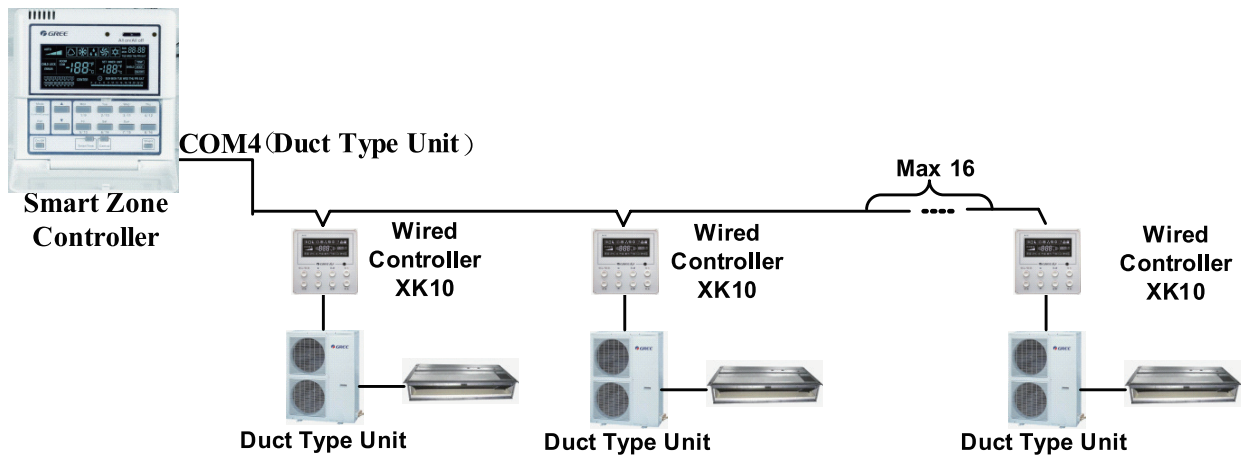
Network Connection of the Smart Zone Controller
