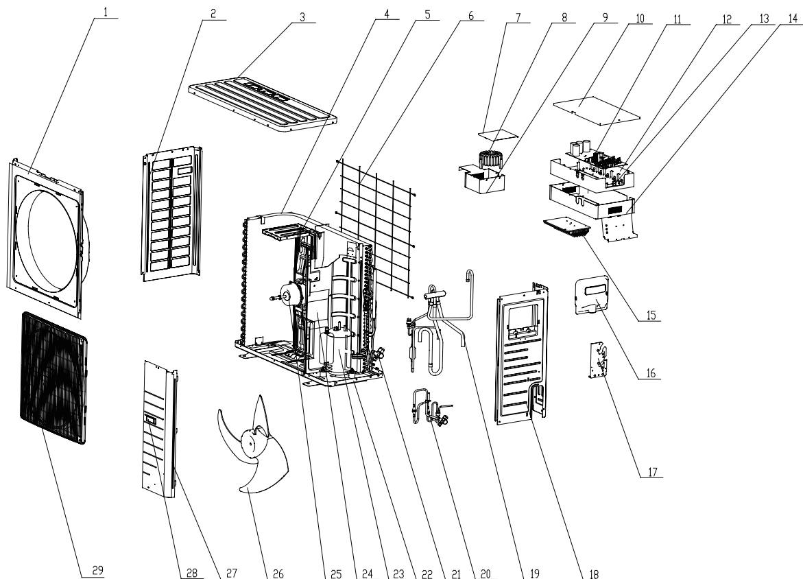
Model: GUHD30NK3CO Exploded View and spare parts list:
